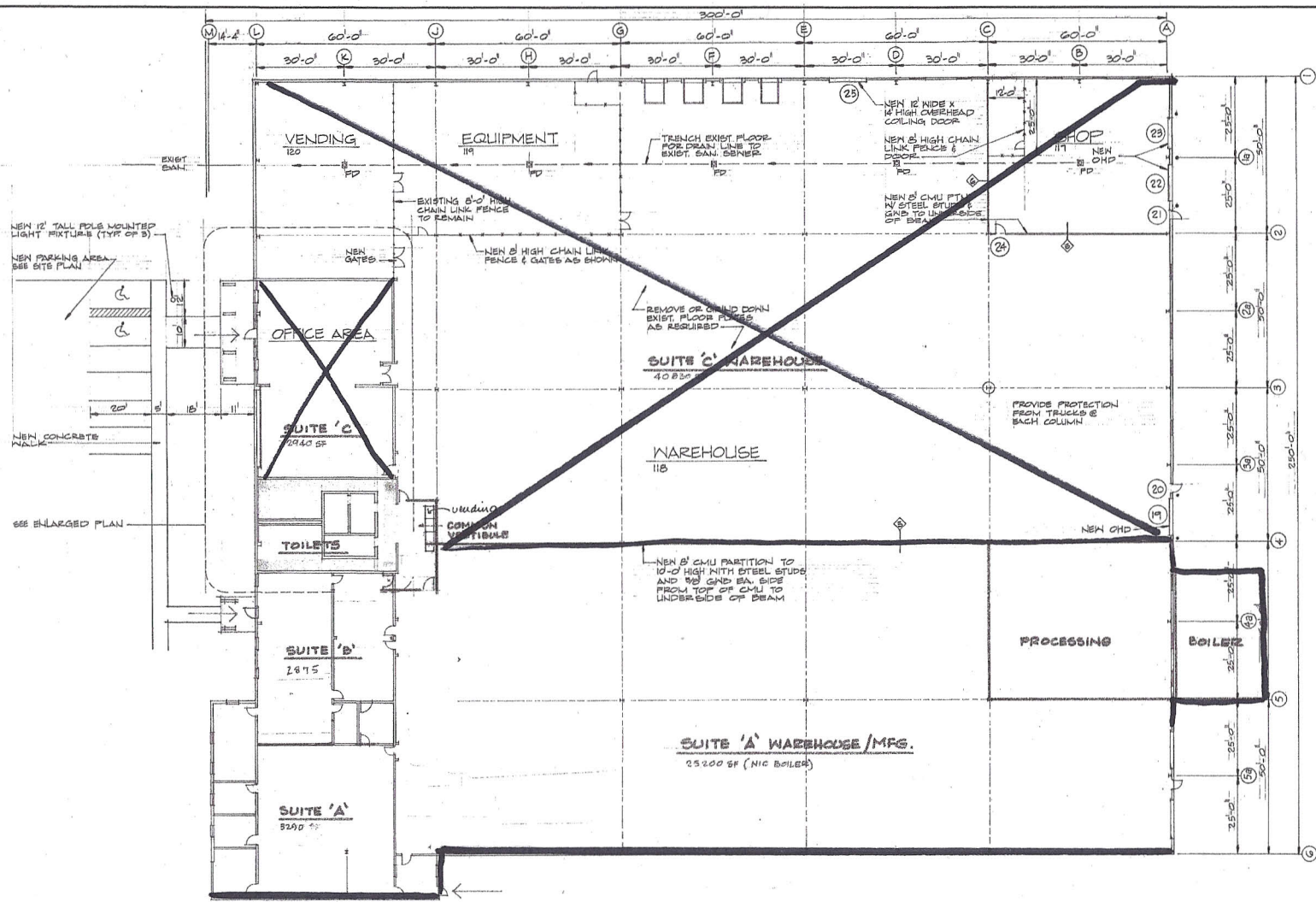
COMPOSITE FLOOR PLAN SCALE 1/8" = 1'-0"
